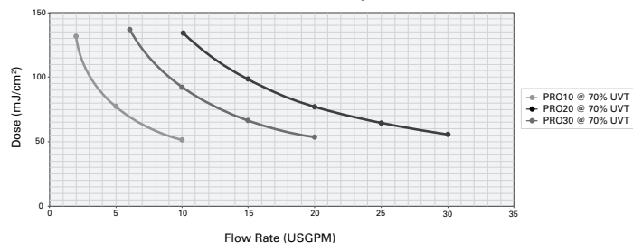
PRO10, PRO20, & PRO30 Dose Response Curves
