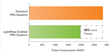
Yearly Power Consumption - 2 x PRO20 Systems
